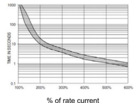
trip time vs. percent of rated current
